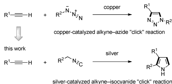
Scheme 1. Proposed click synthesis of pyrroles.
