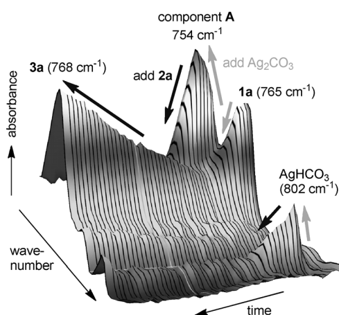
Figure 1. Profile of the stepwise stoichiometric reaction between 1a , Ag 2 CO 3 , and 2a in DMSO at 80 °C monitored by in situ IR spectroscopy.
