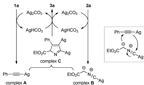
Scheme 4. Proposed mechanism for the silver-catalyzed cycloaddition of terminal alkynes with isocyanides.
