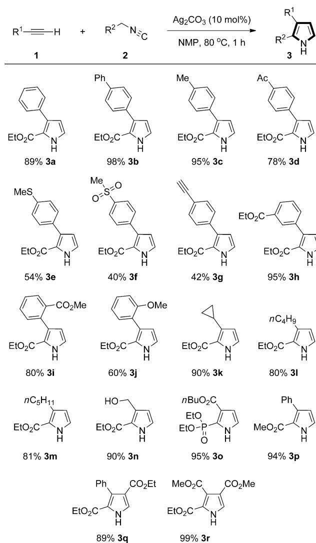
Scheme 2. Cycloaddition of alkynes 1 and isocyanides 2 . Reaction conditions: 1 (0.5 mmol), 2 (0.75 mmol), Ag 2 CO 3 (10 mol%) in 2 mL of NMP at 80 °C under N 2 atmosphere for 1 h. Yields of isolated products are given.
