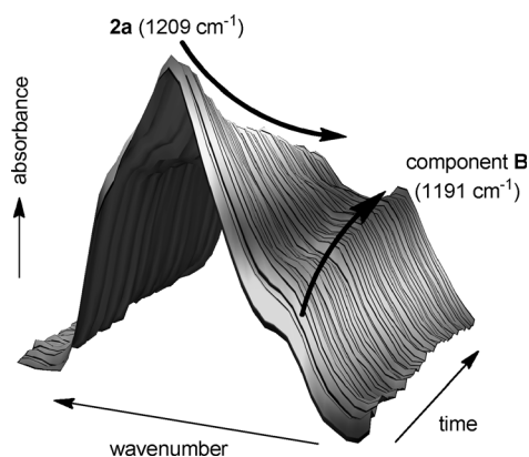
Figure 2. Profile of the stoichiometric reaction between 2a and \text{Ag}_2\text{CO}_3 in DMSO at 80^\circ\text{C} monitored by in situ IR spectroscopy.
